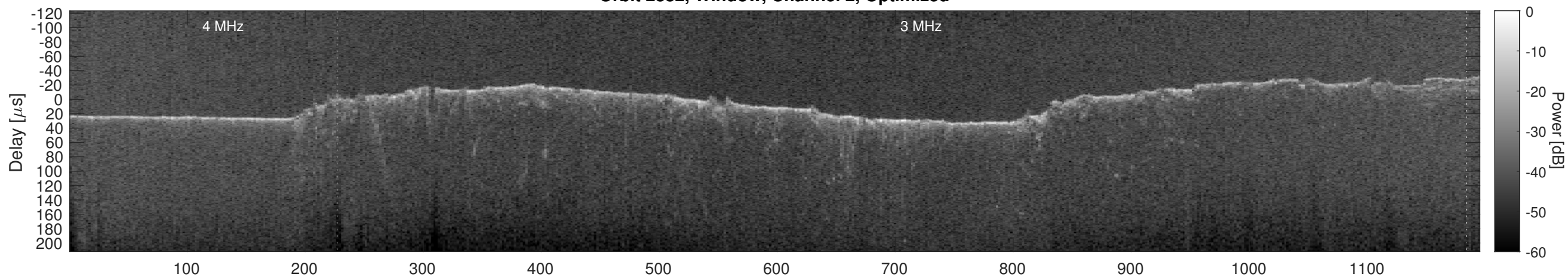
Orbit 2882, Cluttergram
