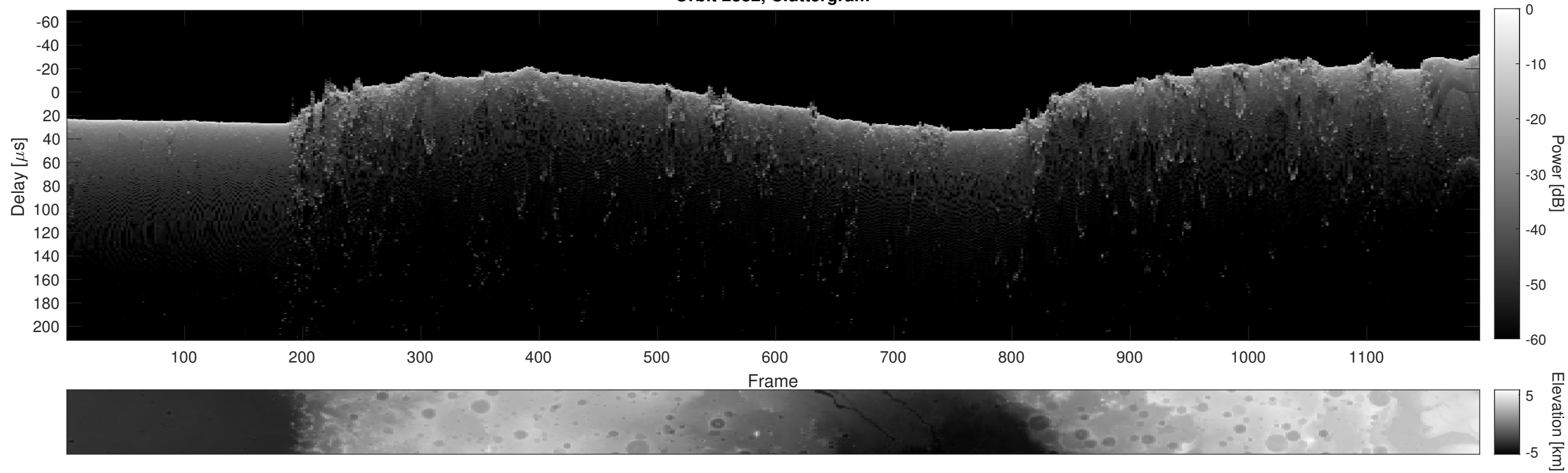
Orbit 2882, Cluttergram
