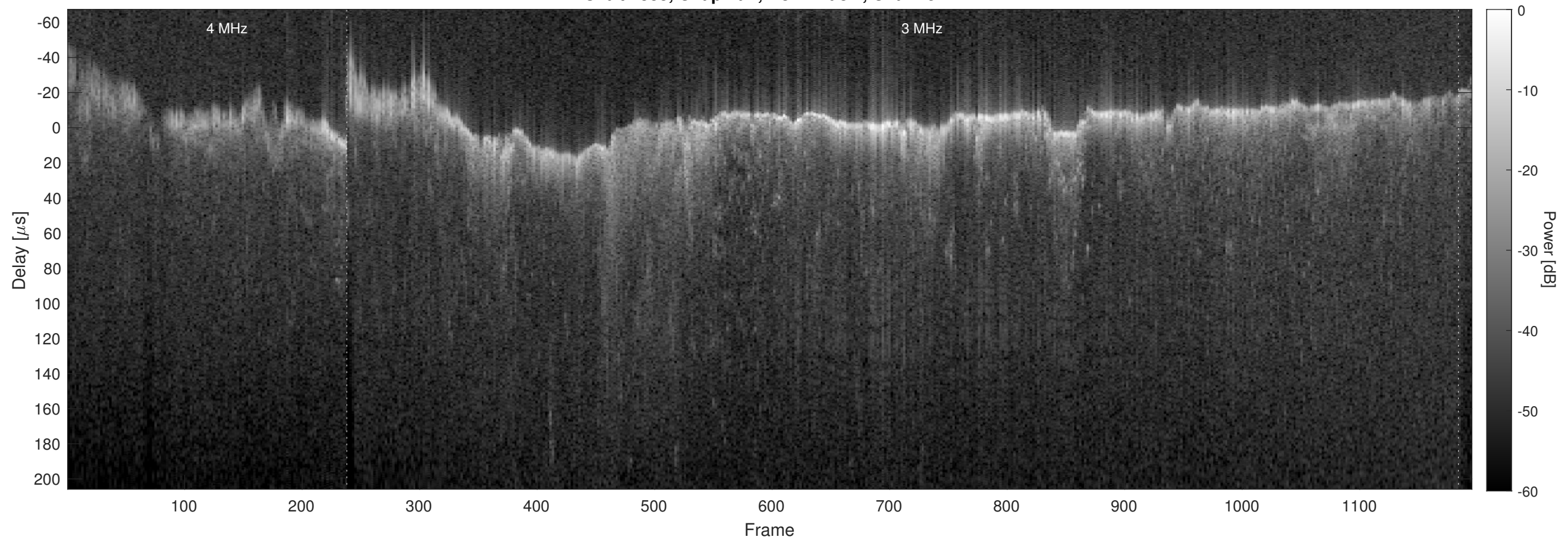
Orbit 2883, Chapman, No Window, Channel 2
