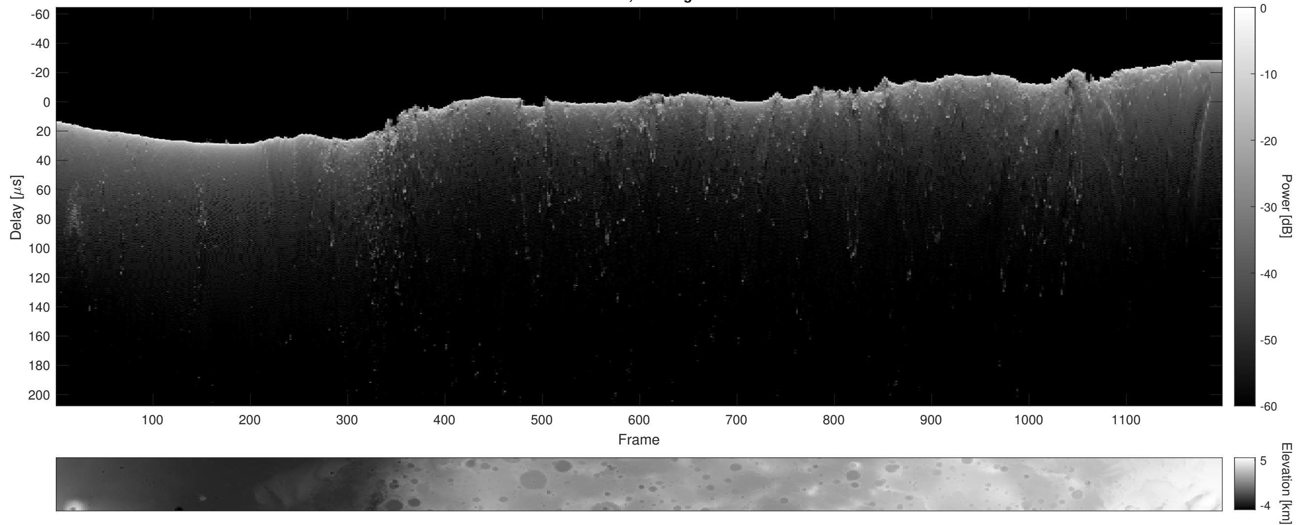
Orbit 2885, Cluttergram
