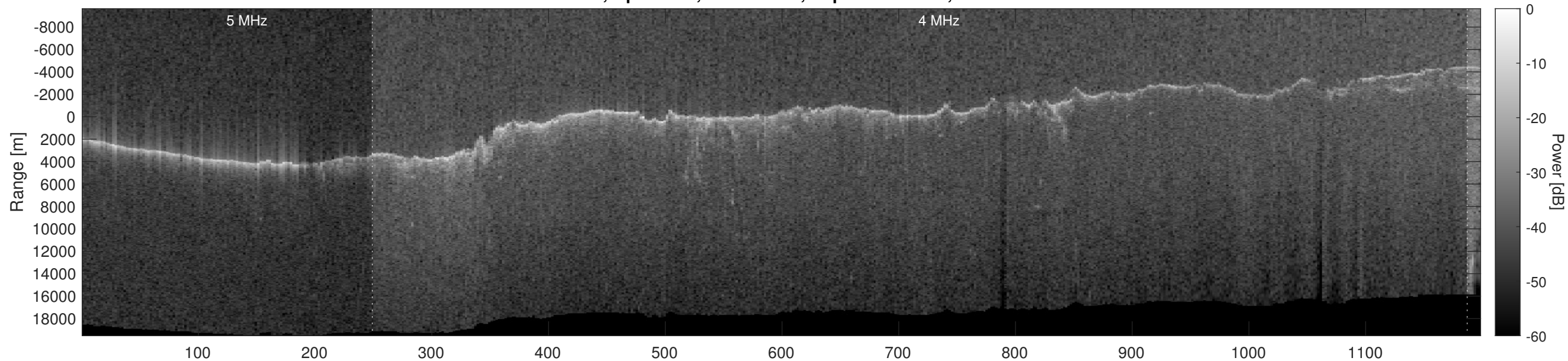
Orbit 2885, Optimized, No Window, Depth-Corrected, Channel 2
