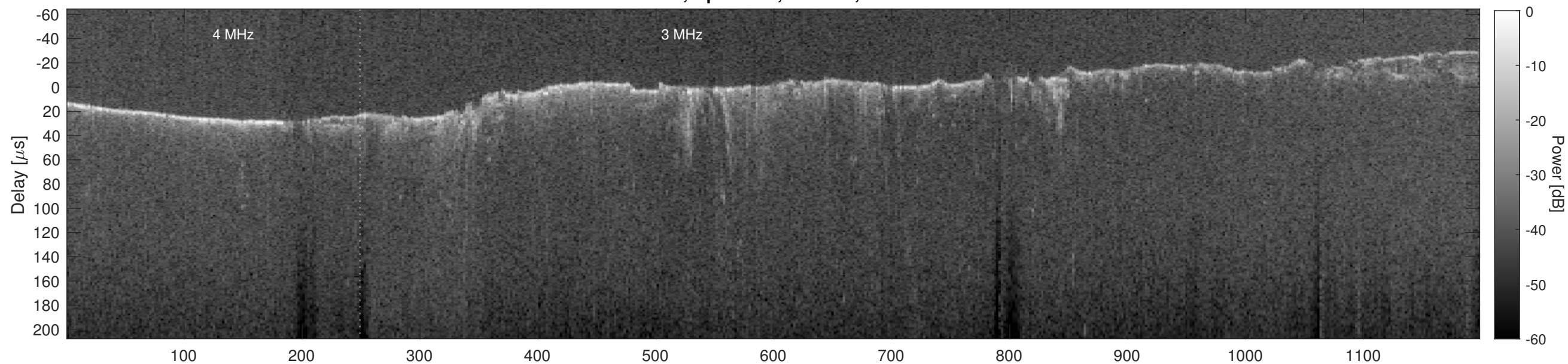
Orbit 2885, Cluttergram
