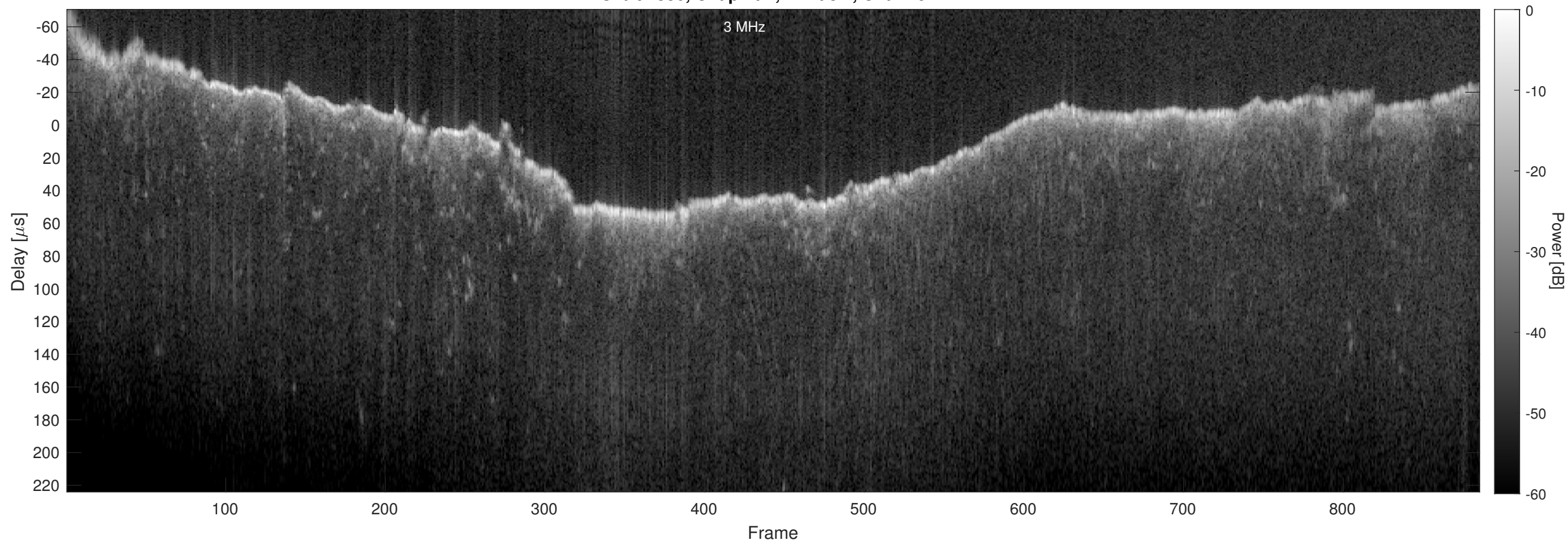
Orbit 2886, Chapman, Window, Channel 2
