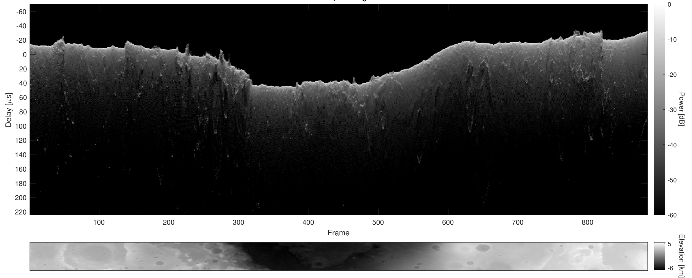
Orbit 2886, Cluttergram
