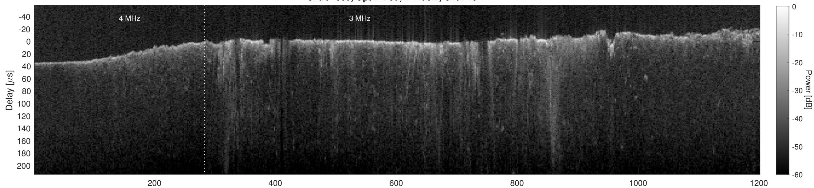
Orbit 2889, Cluttergram
