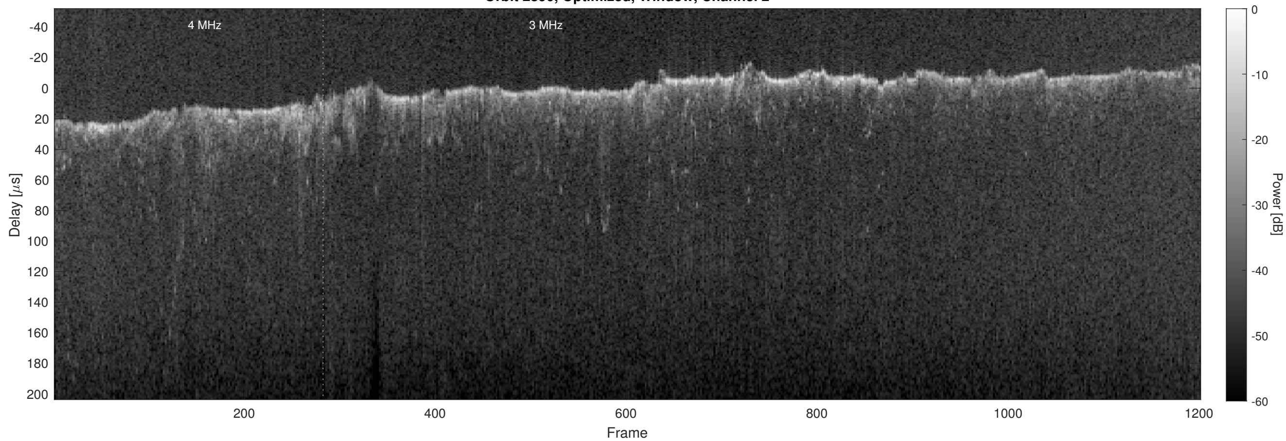
Orbit 2890, Optimized, Window, Channel 2
