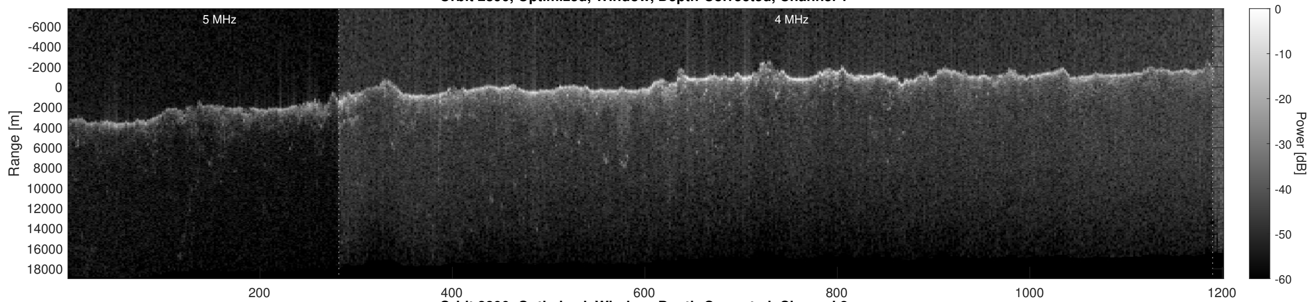
Orbit 2890, Optimized, Window, Depth-Corrected, Channel 2
