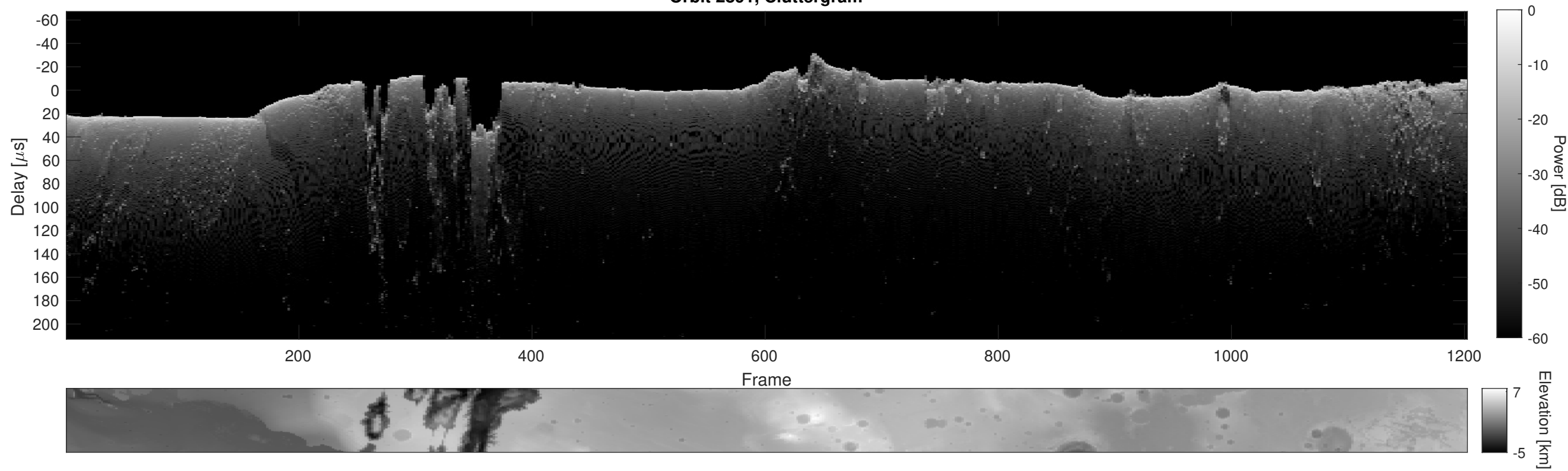
Orbit 2891, Cluttergram
