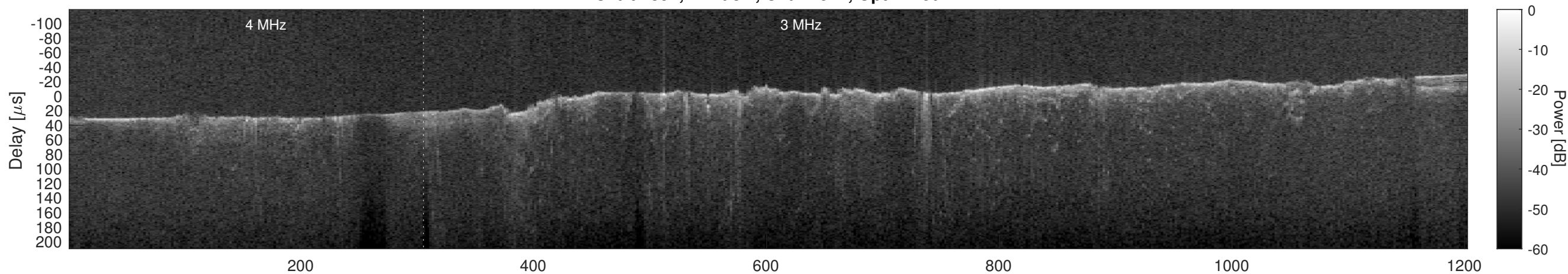
Orbit 2892, Cluttergram
