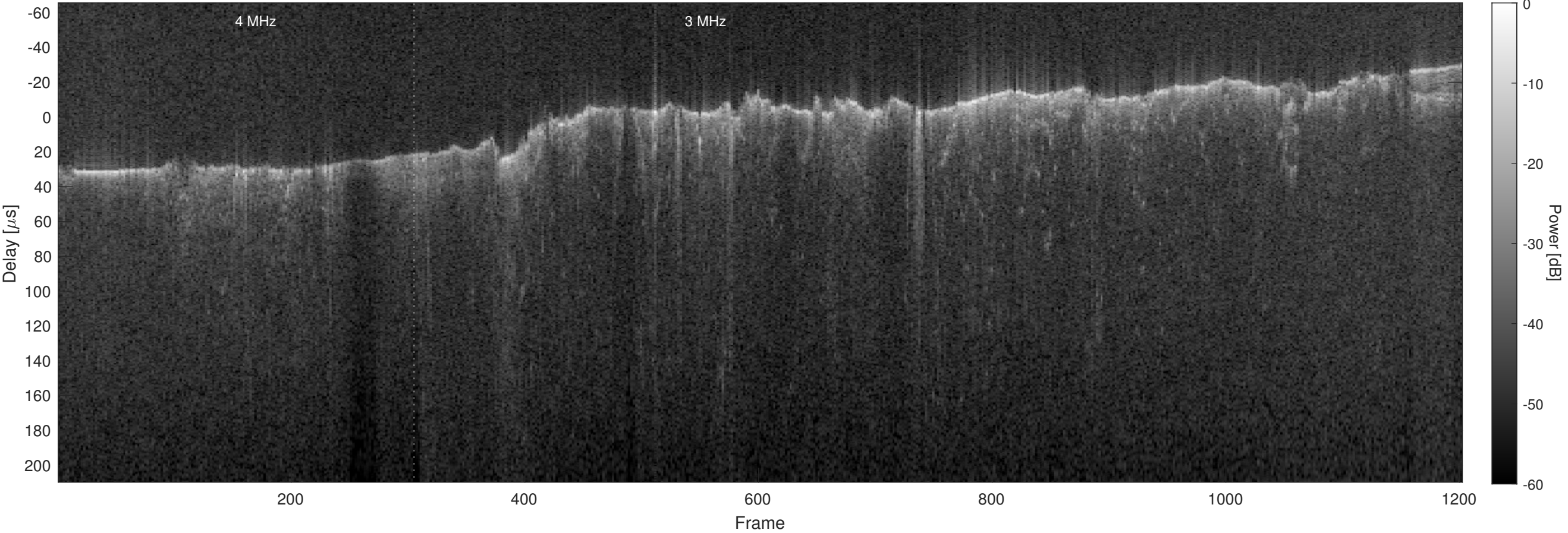
Orbit 2892, Optimized, No Window, Channel 2
