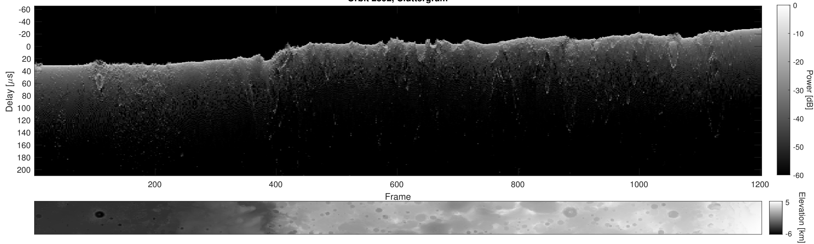
Orbit 2892, Cluttergram
