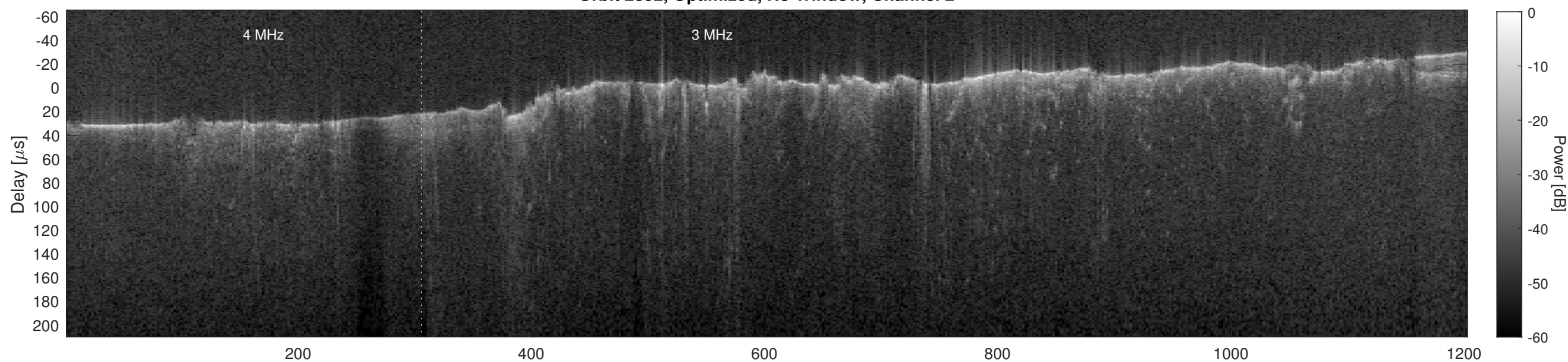
Orbit 2892, Cluttergram
