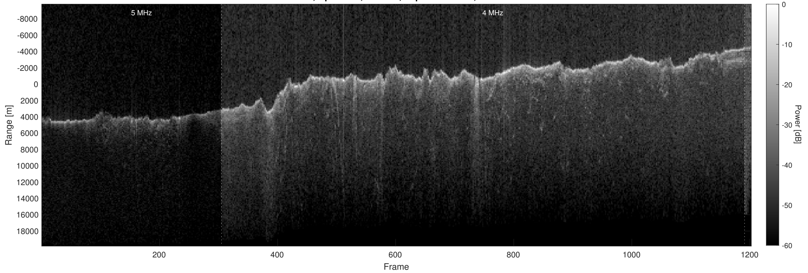
Orbit 2892, Optimized, Window, Depth-Corrected, Channel 2
