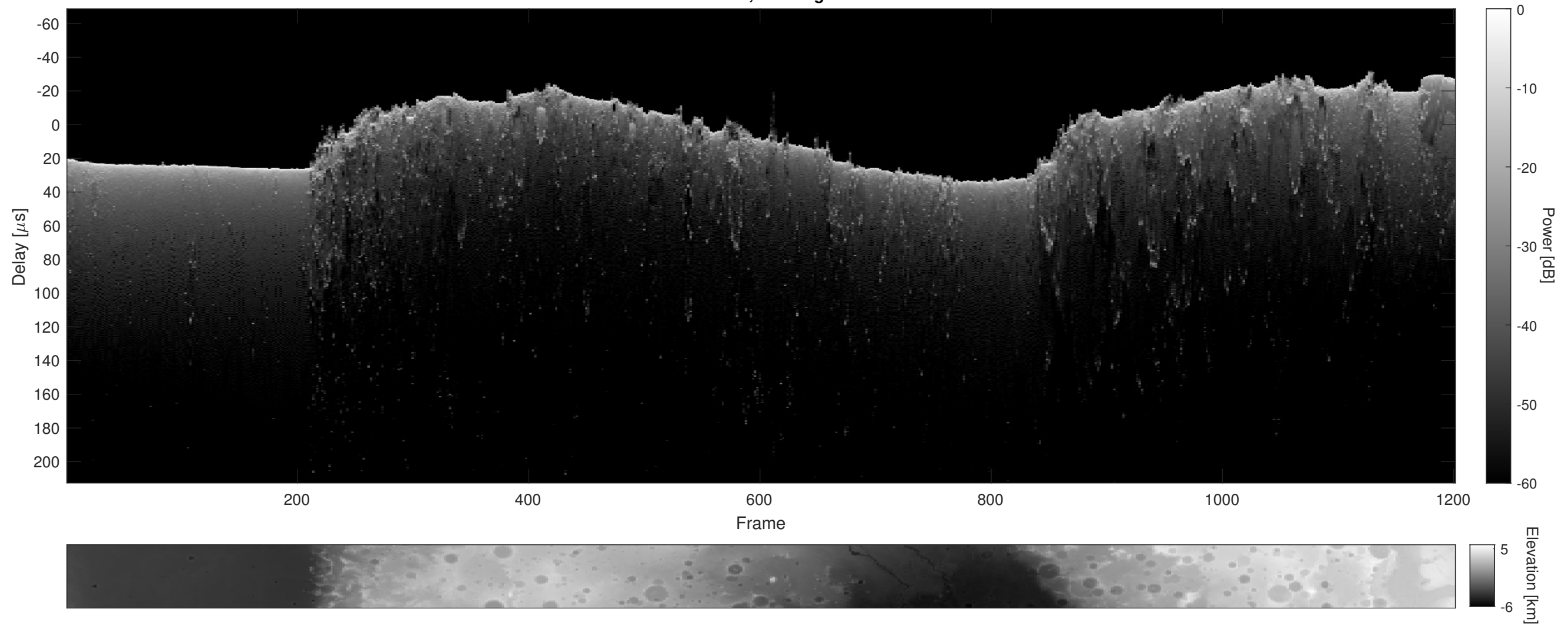
Orbit 2893, Cluttergram
