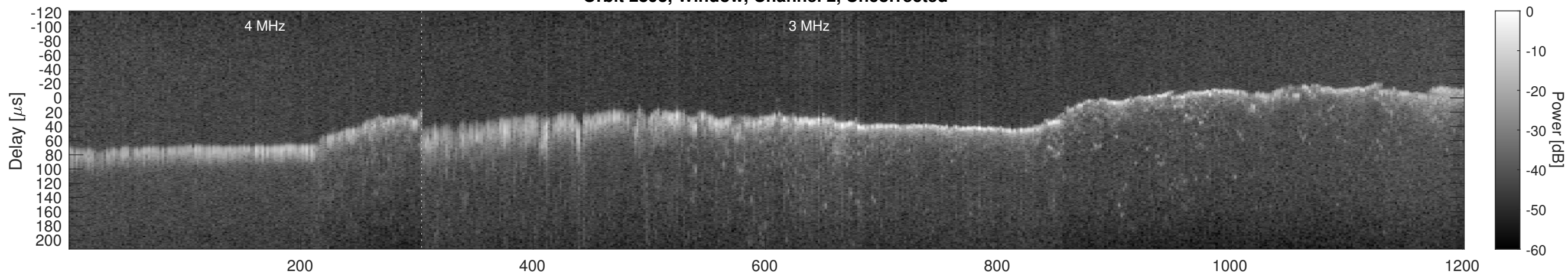
Orbit 2893, Window, Channel 2, Chapman
