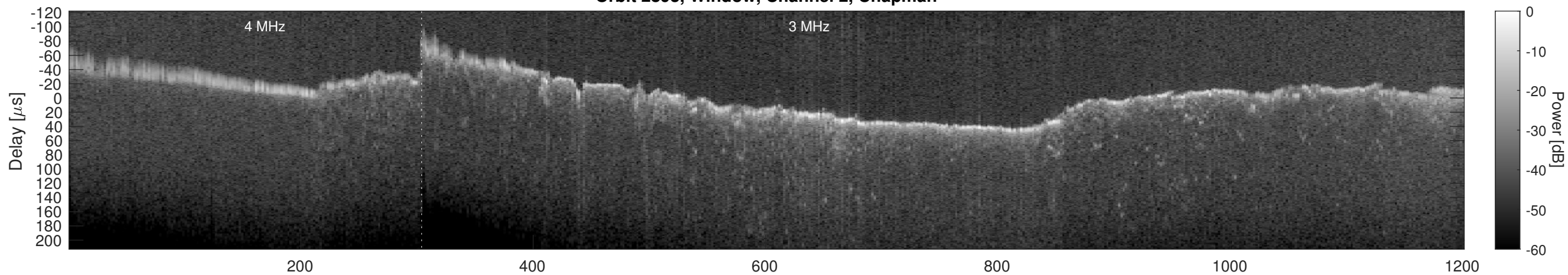
Orbit 2893, Window, Channel 2, Optimized
