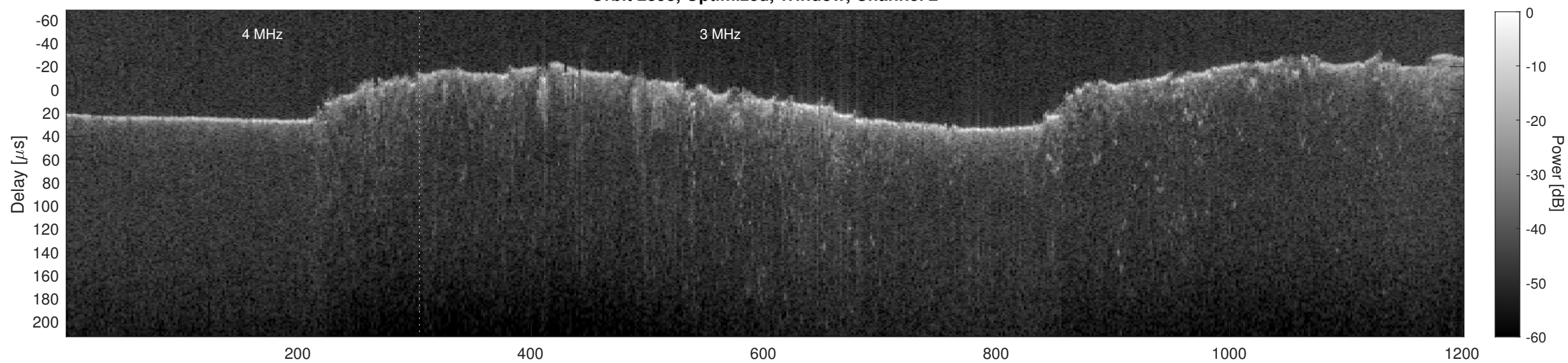
Orbit 2893, Cluttergram
