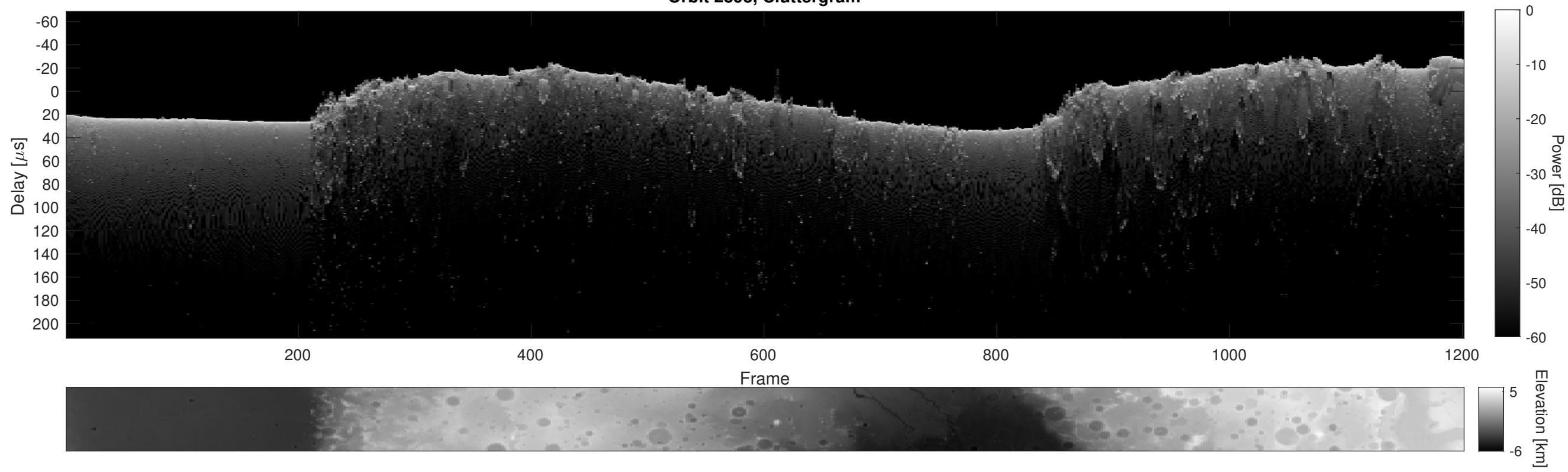
Orbit 2893, Cluttergram
