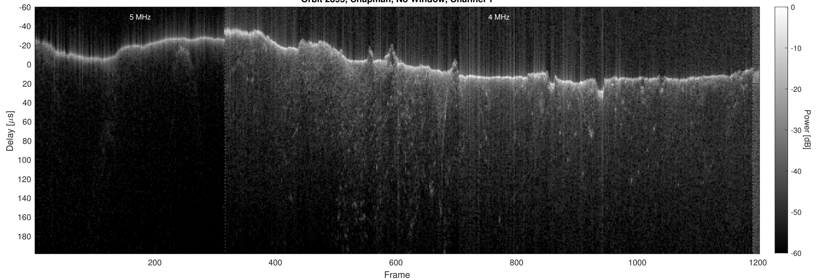
Orbit 2895, Chapman, No Window, Channel 2
