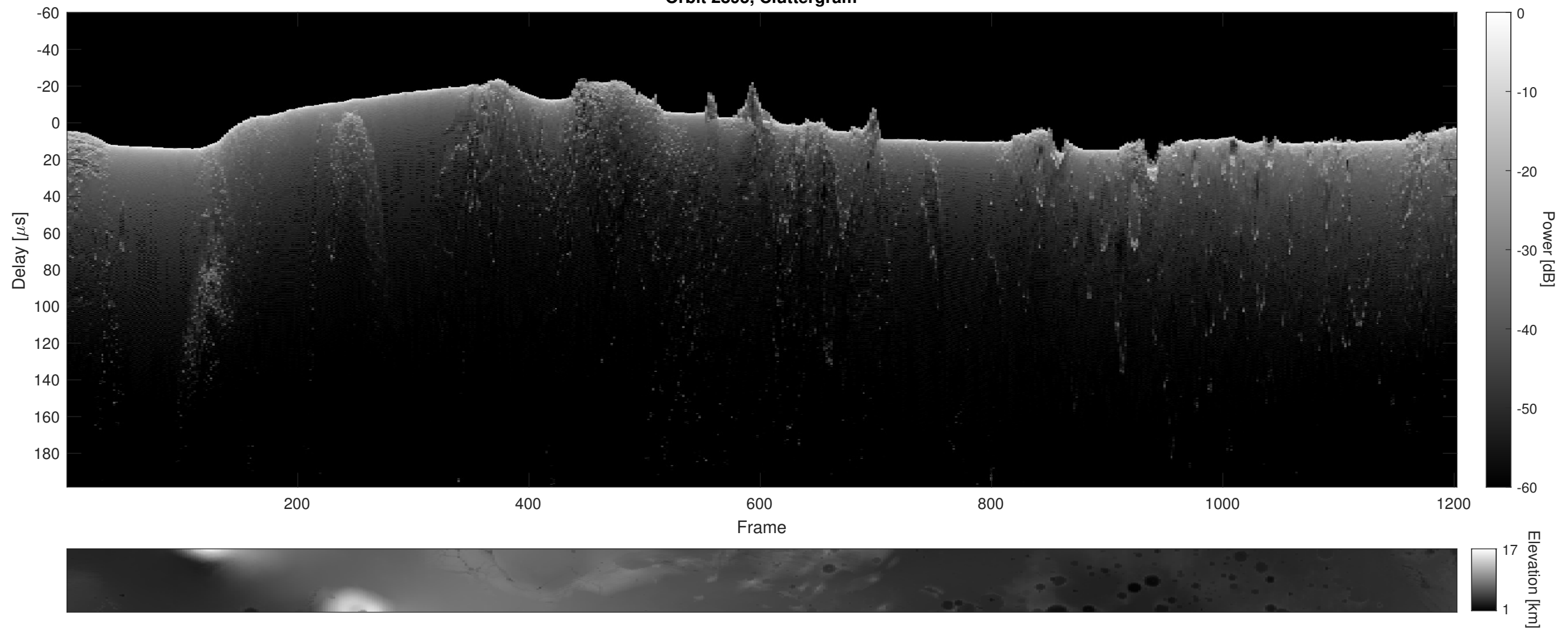
Orbit 2895, Cluttergram
