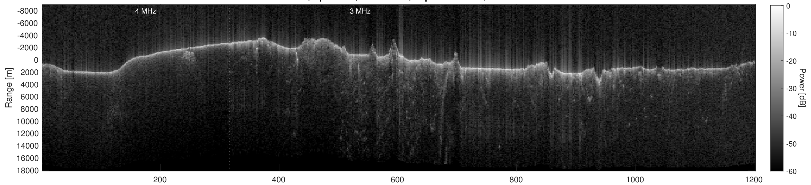
Orbit 2895, Depth-Corrected Cluttergram
