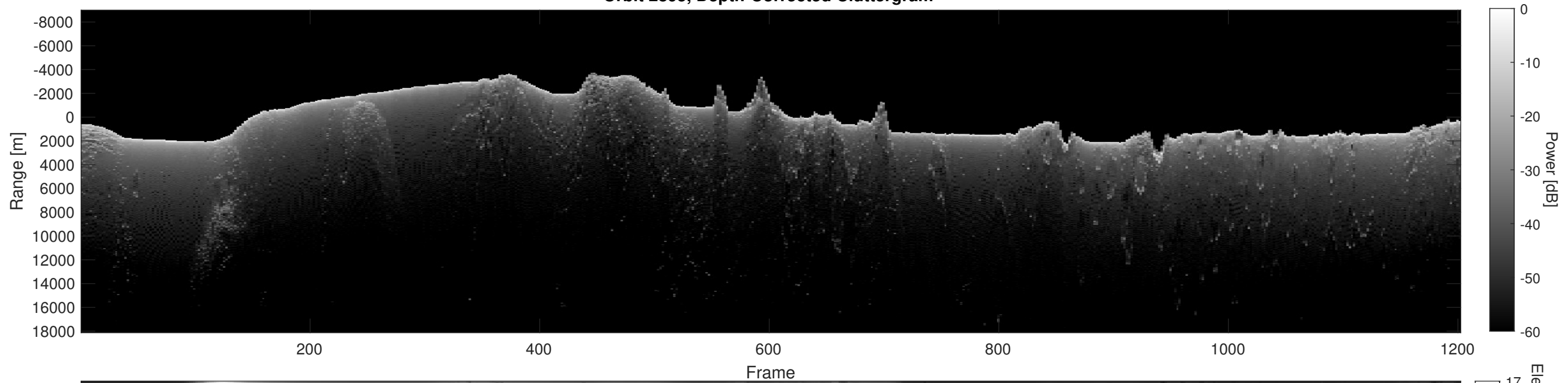
Orbit 2895, Depth-Corrected Cluttergram
