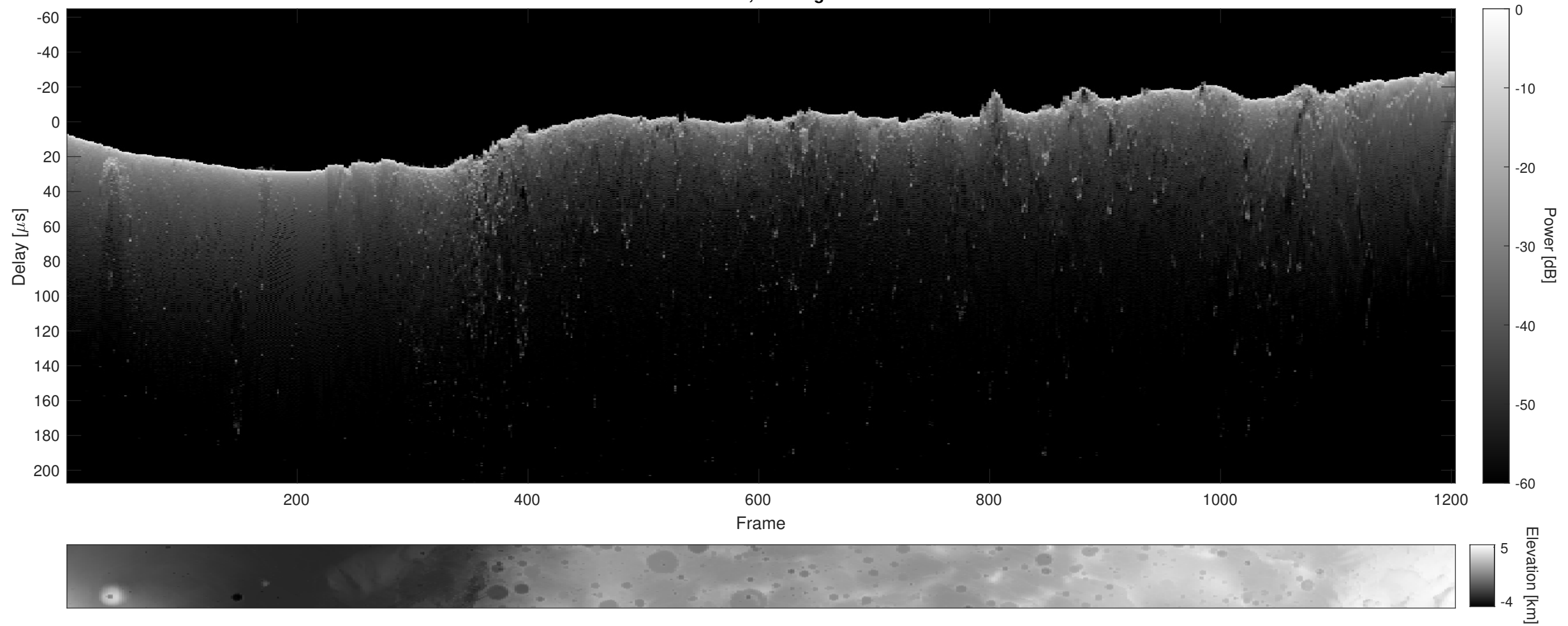
Orbit 2896, Cluttergram
