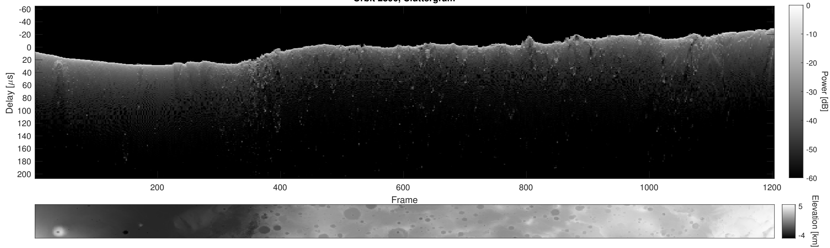
Orbit 2896, Cluttergram
