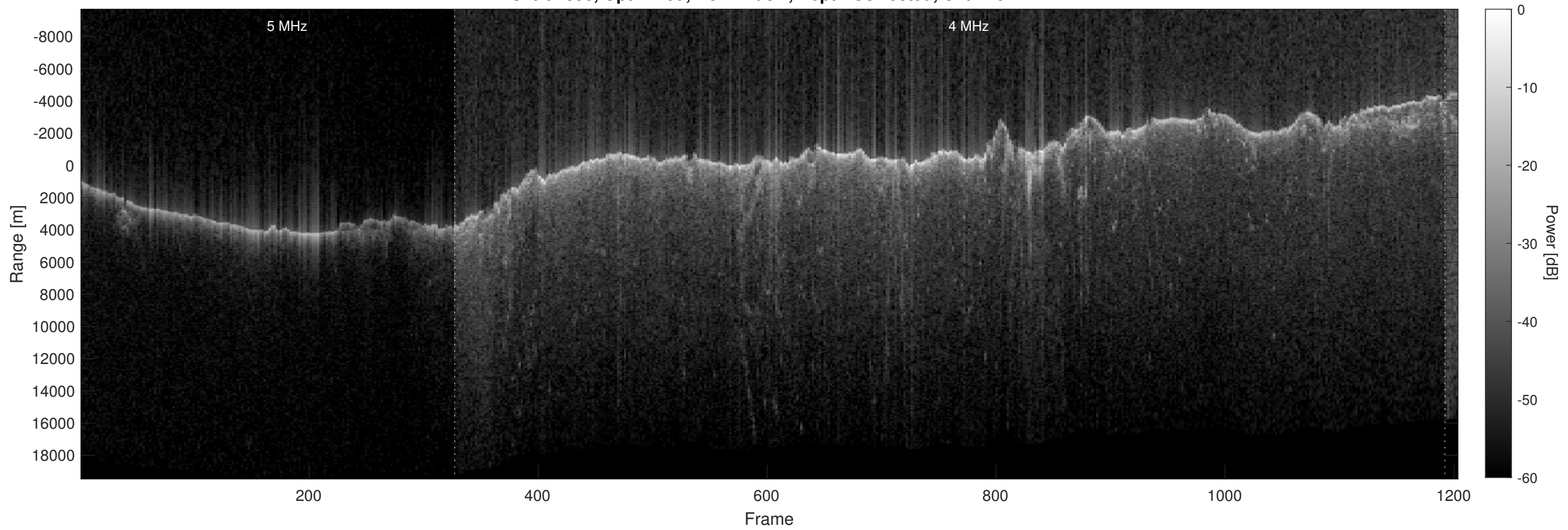
Orbit 2896, Optimized, No Window, Depth-Corrected, Channel 2
