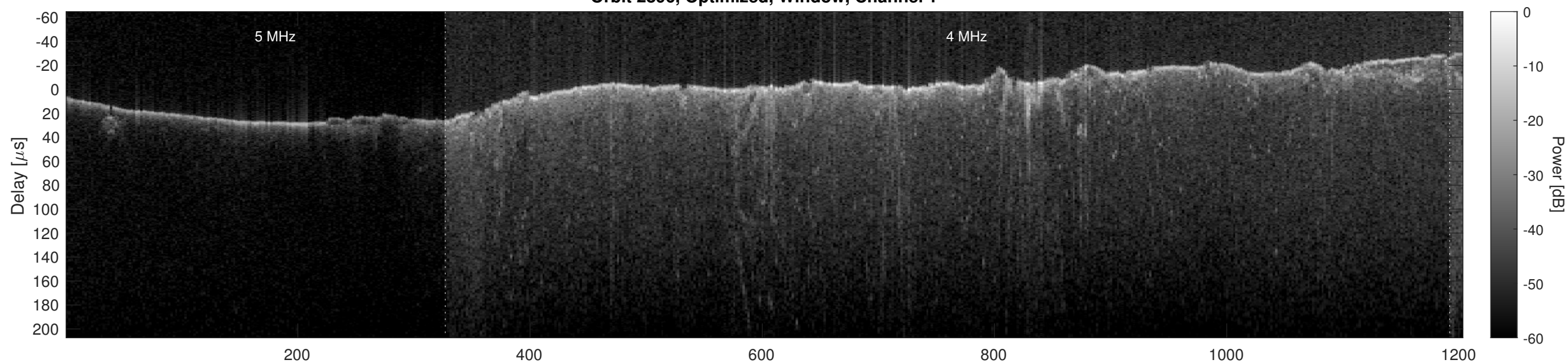
Orbit 2896, Optimized, Window, Channel 2
