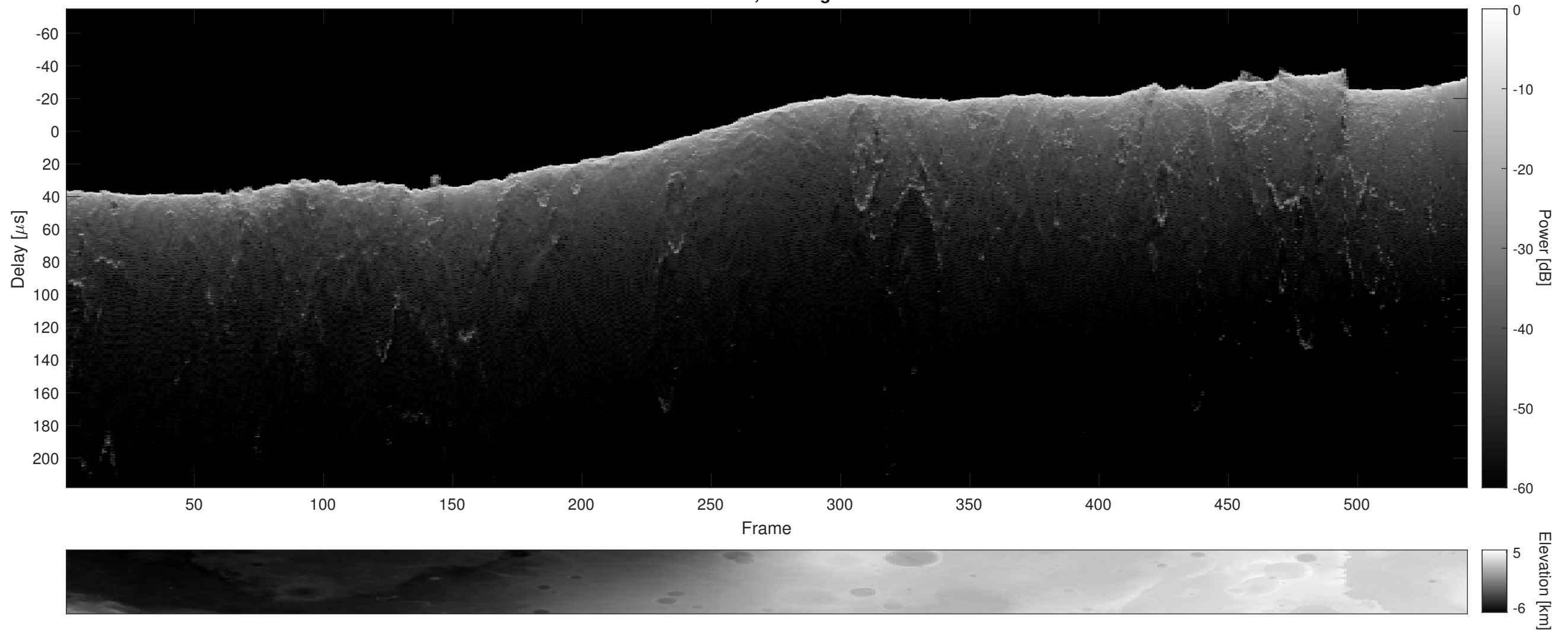
Orbit 2897, Cluttergram
