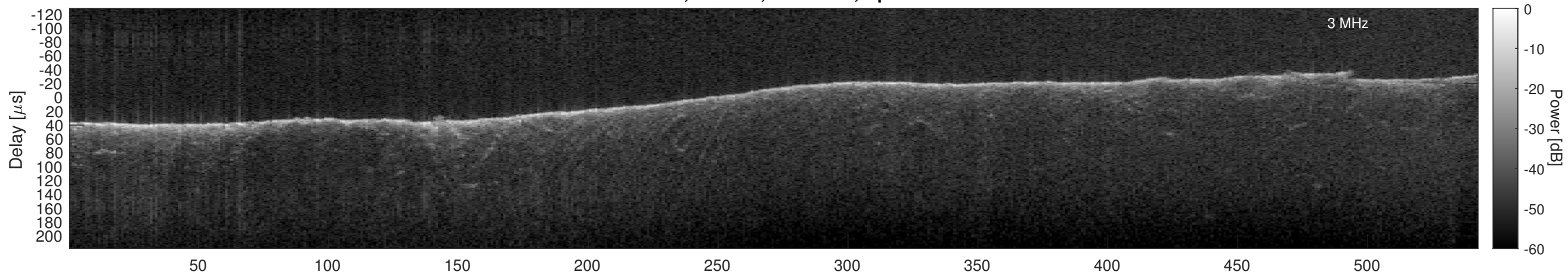
Orbit 2897, Cluttergram
