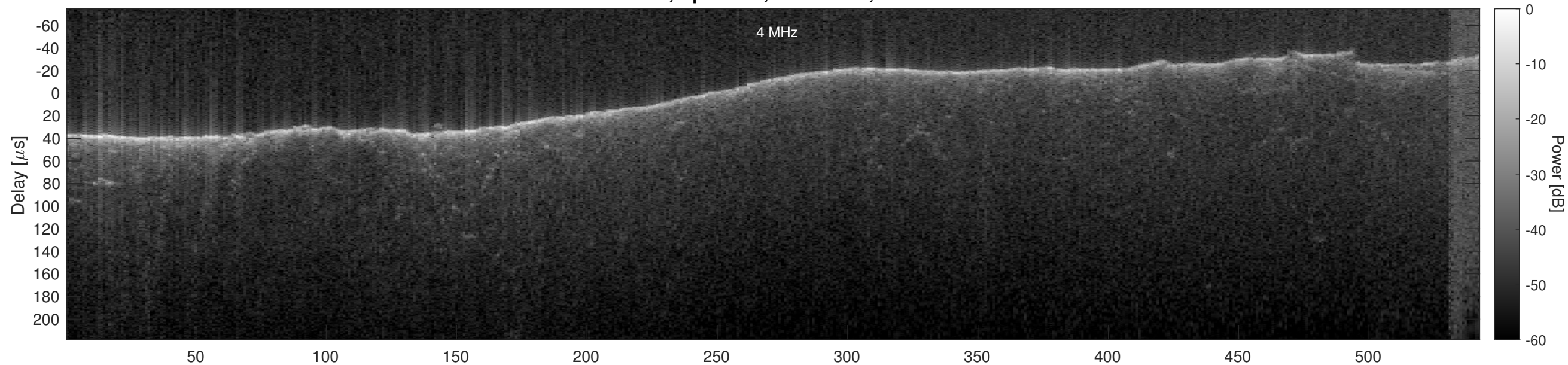
Orbit 2897, Optimized, No Window, Channel 2
