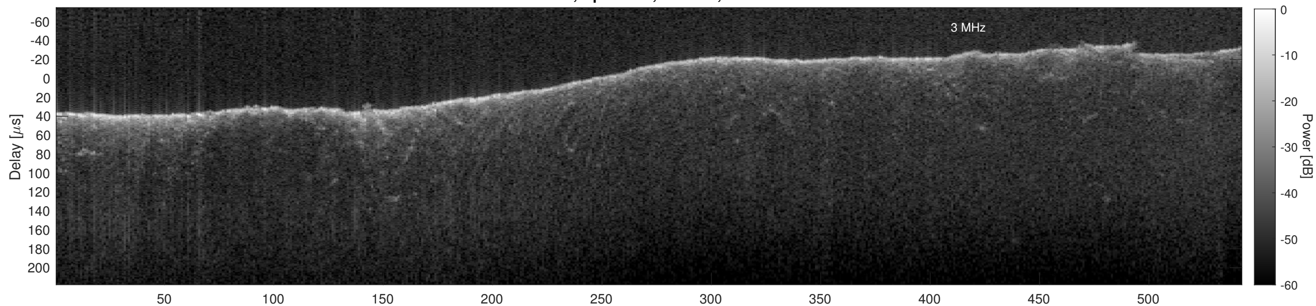
Orbit 2897, Cluttergram
