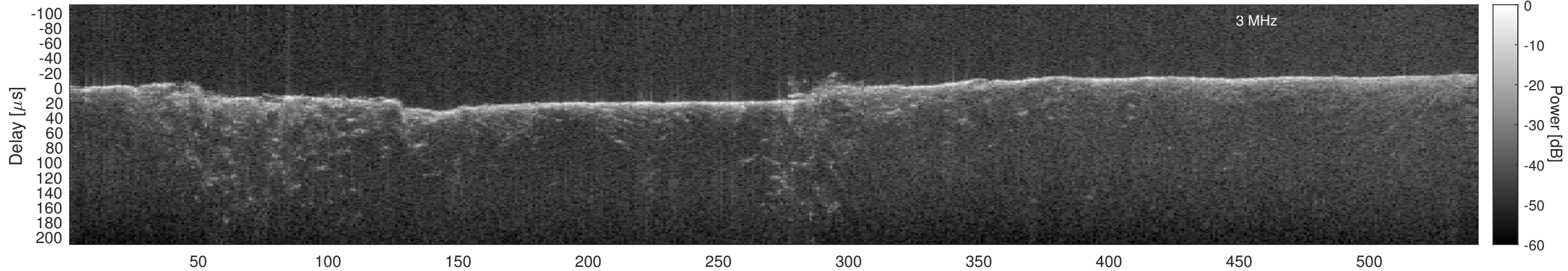
Orbit 2898, Cluttergram
