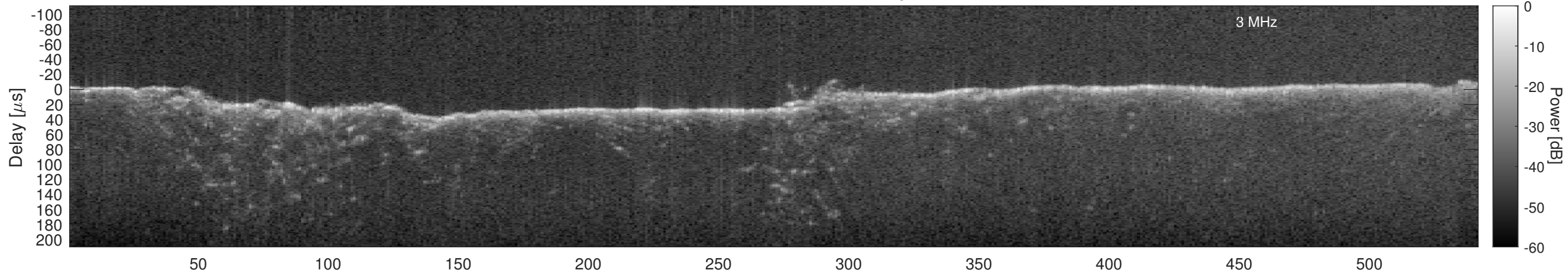
Orbit 2898, Window, Channel 2, Optimized
