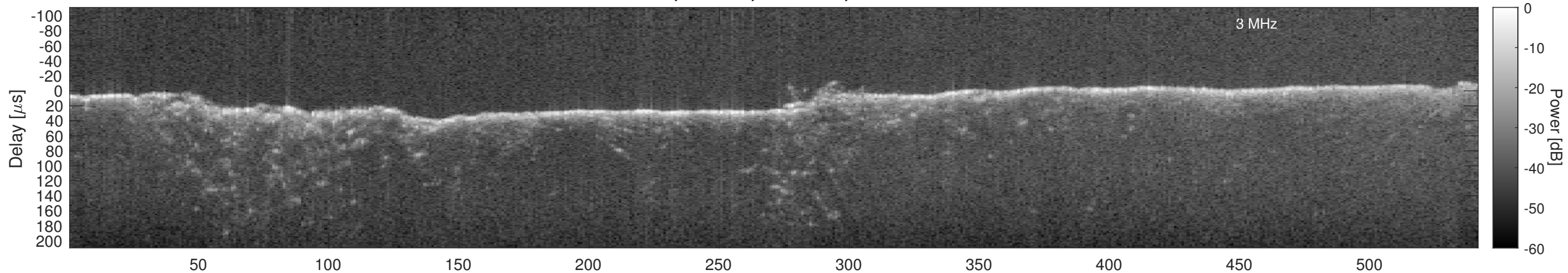
Orbit 2898, Window, Channel 2, Chapman
