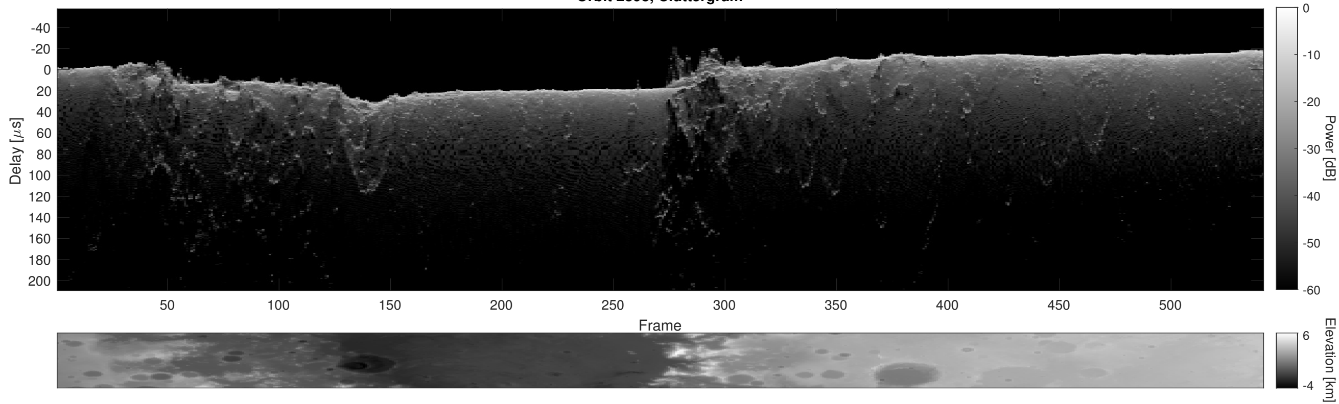
Orbit 2898, Cluttergram
