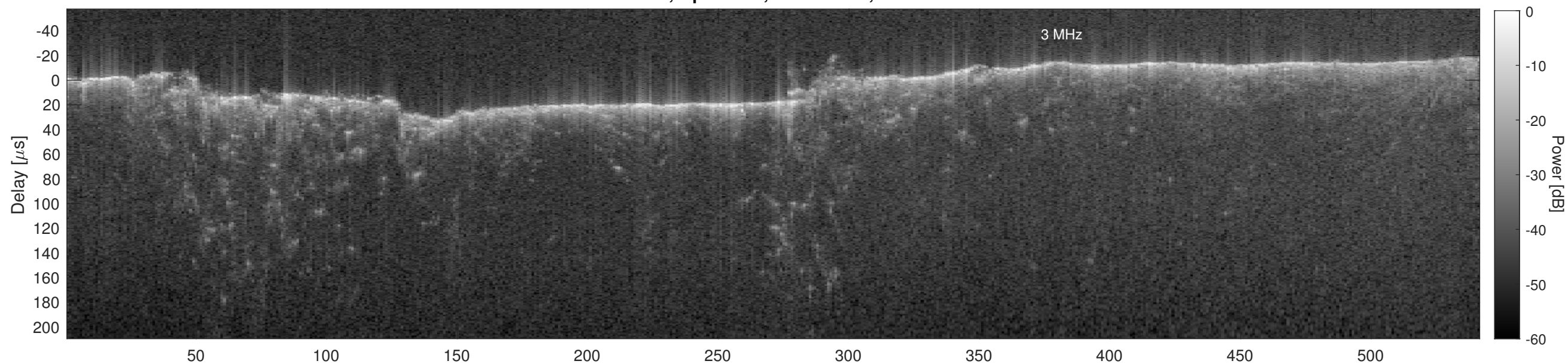
Orbit 2898, Cluttergram
