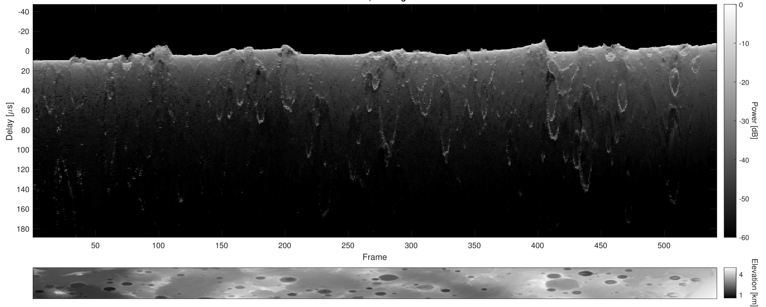
Orbit 2899, Cluttergram
