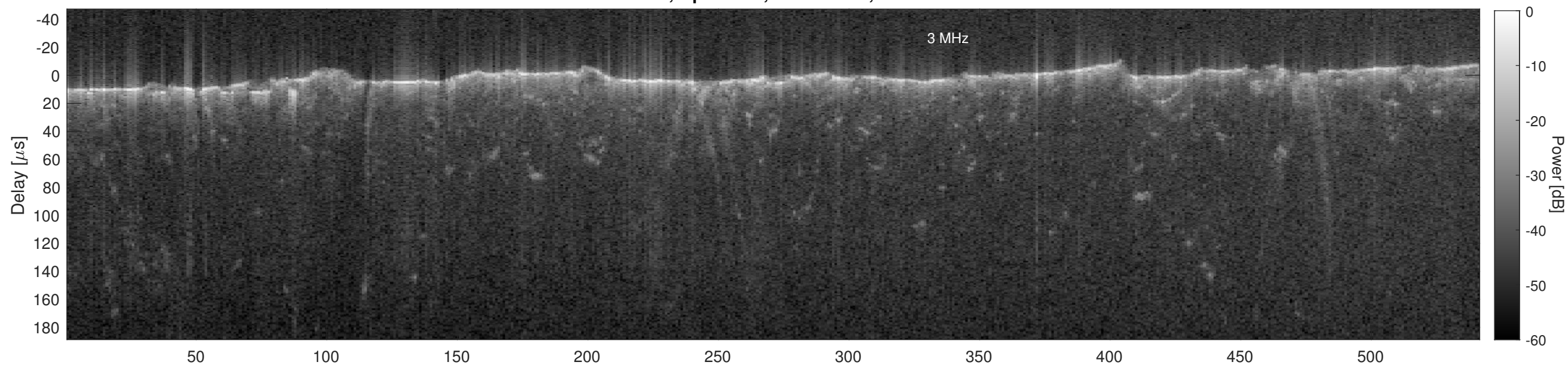
Orbit 2899, Cluttergram
