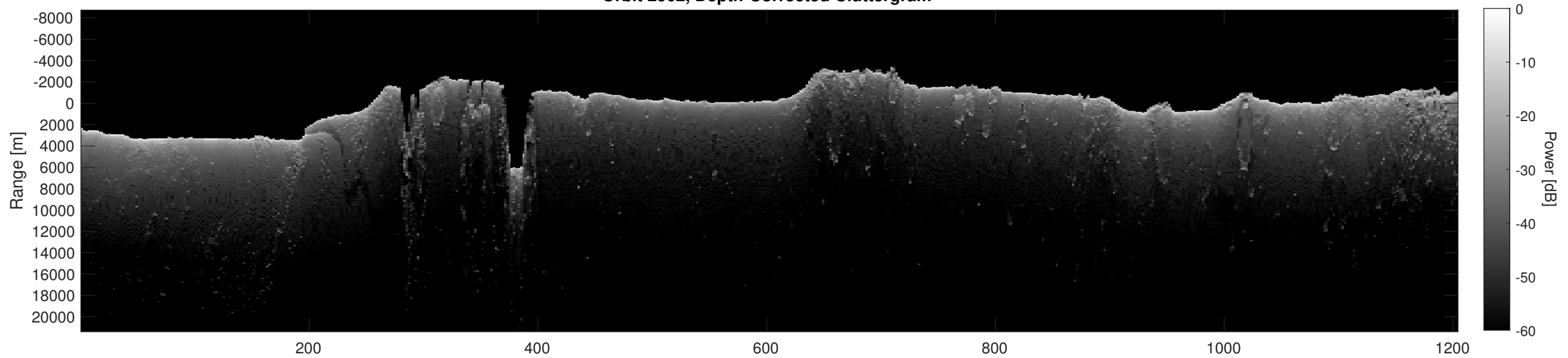
Orbit 2902, Depth-Corrected Cluttergram
