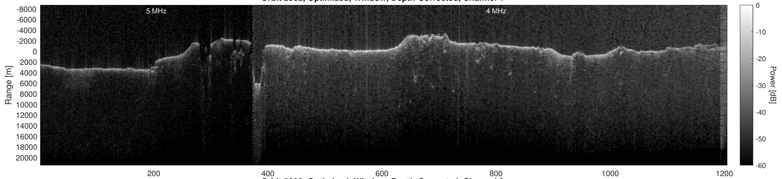
Orbit 2902, Optimized, Window, Depth-Corrected, Channel 2
