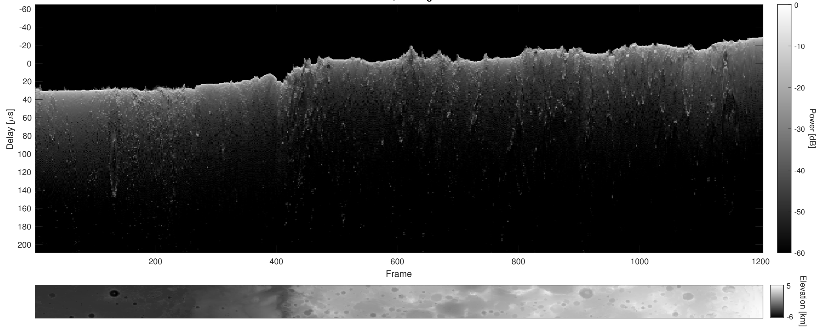
Orbit 2903, Cluttergram
