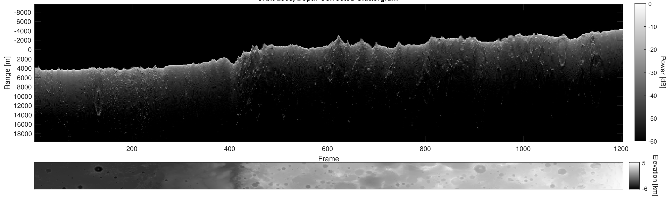
Orbit 2903, Depth-Corrected Cluttergram
