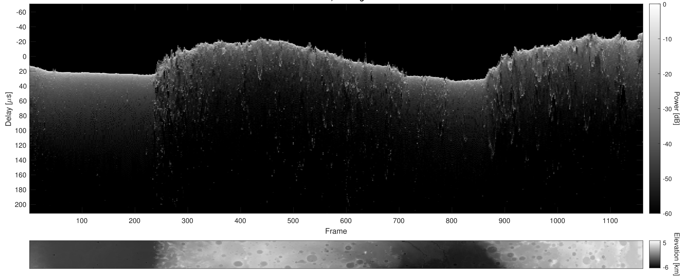
Orbit 2904, Cluttergram
