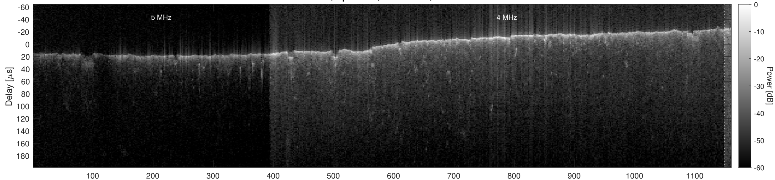
Orbit 2905, Optimized, No Window, Channel 2
