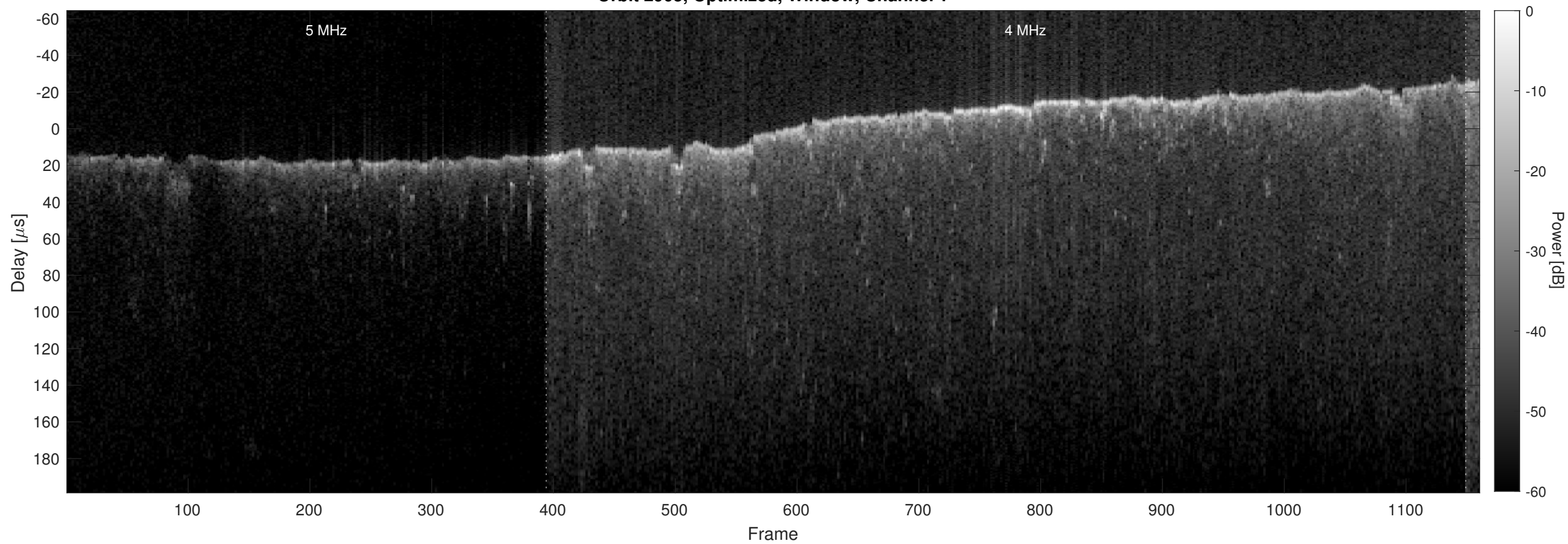
Orbit 2905, Optimized, Window, Channel 2
