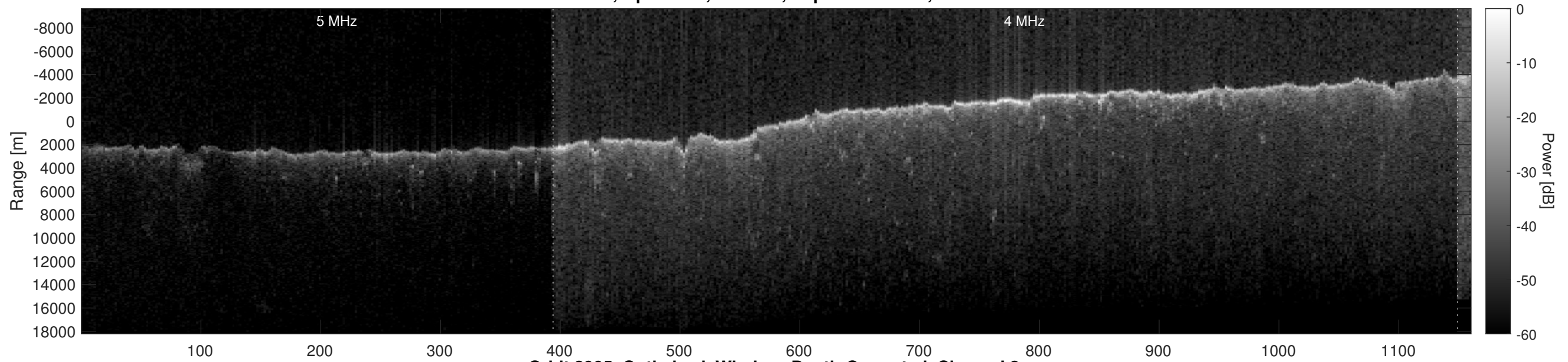
Orbit 2905, Optimized, Window, Depth-Corrected, Channel 2
