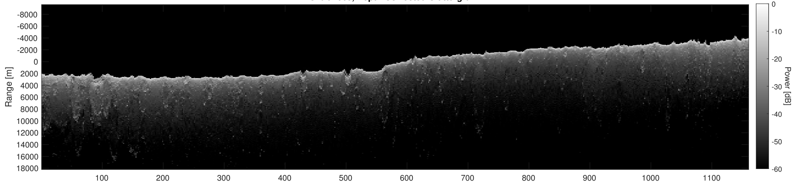
Orbit 2905, Depth-Corrected Cluttergram
