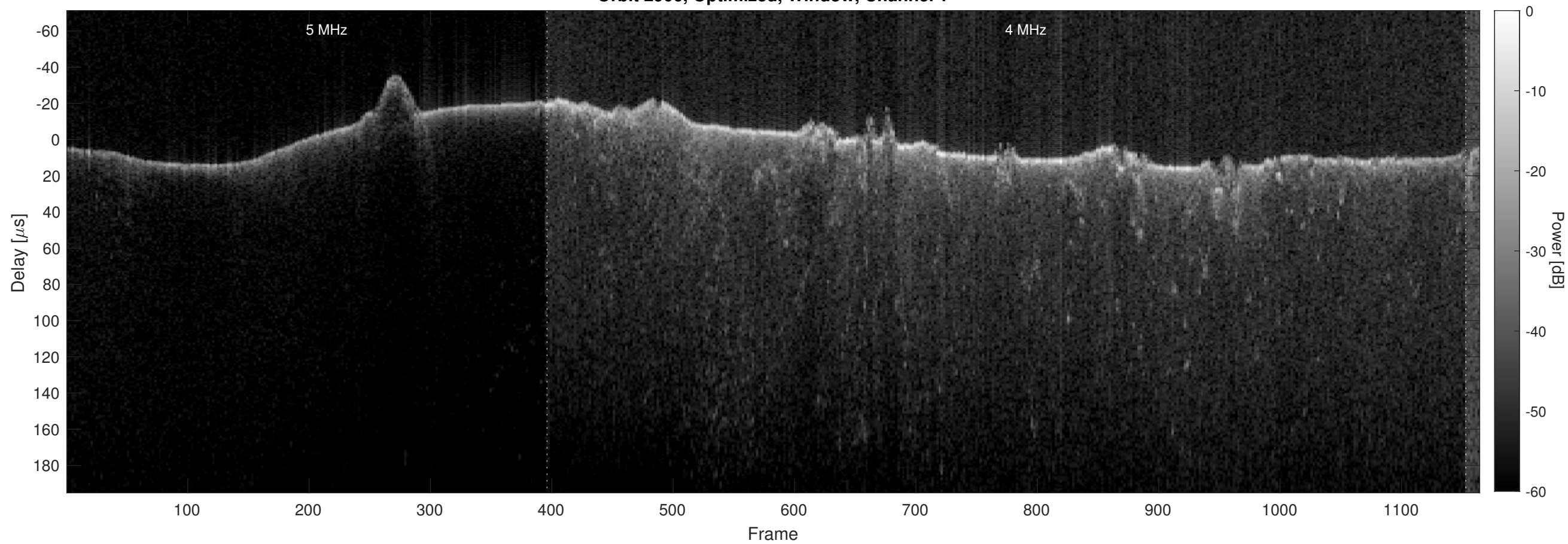
Orbit 2906, Optimized, Window, Channel 2
