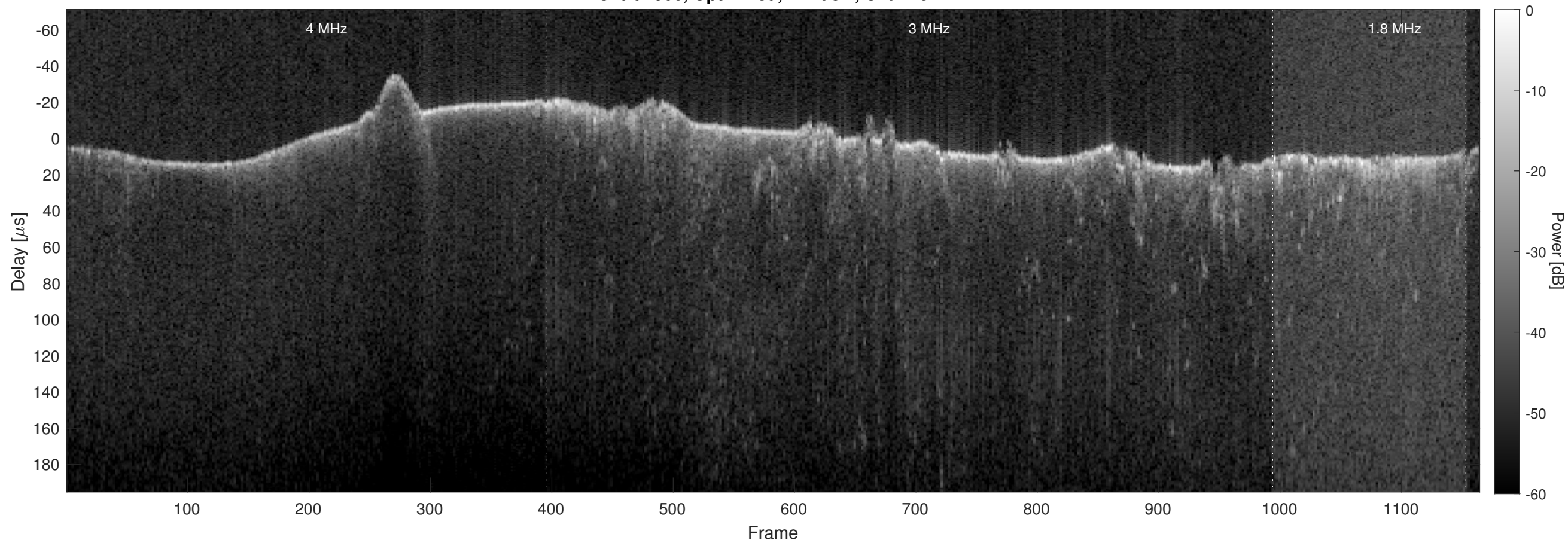
Orbit 2906, Optimized, Window, Channel 2
