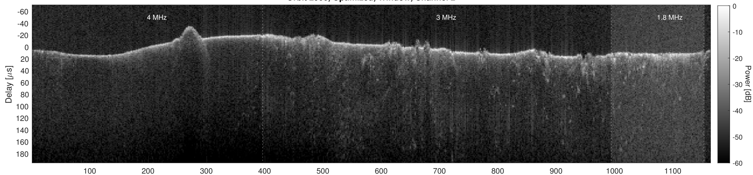
Orbit 2906, Cluttergram
