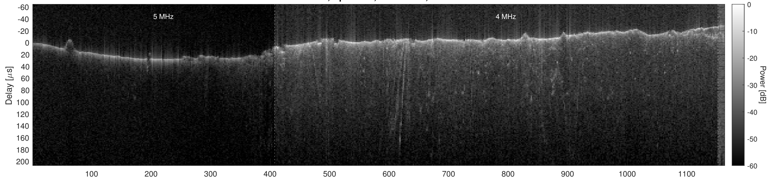
Orbit 2907, Optimized, No Window, Channel 2
