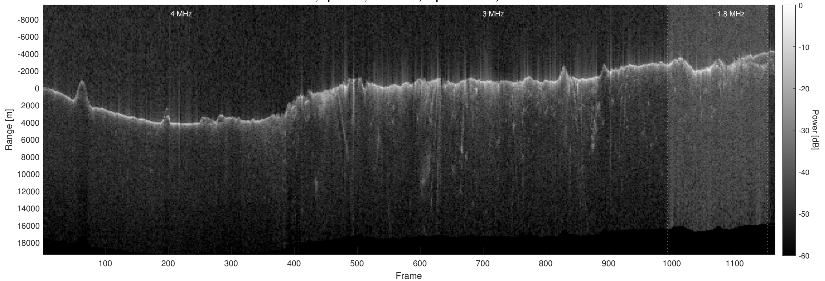
Orbit 2907, Optimized, No Window, Depth-Corrected, Channel 2
