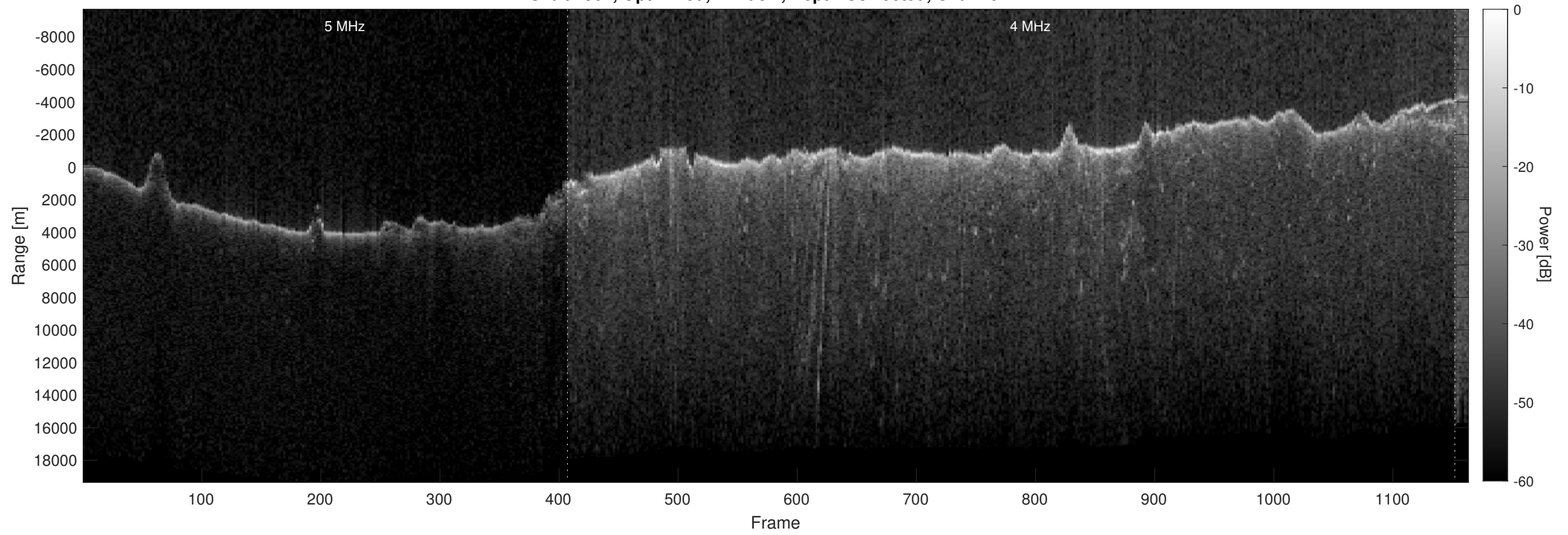
Orbit 2907, Optimized, Window, Depth-Corrected, Channel 2
