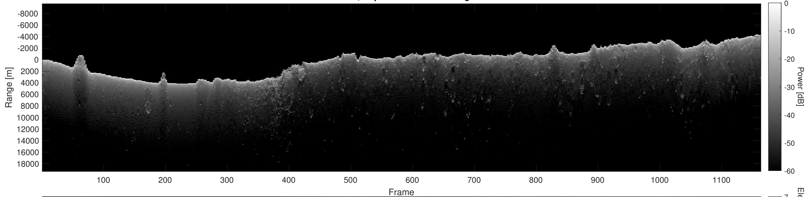
Orbit 2907, Depth-Corrected Cluttergram
