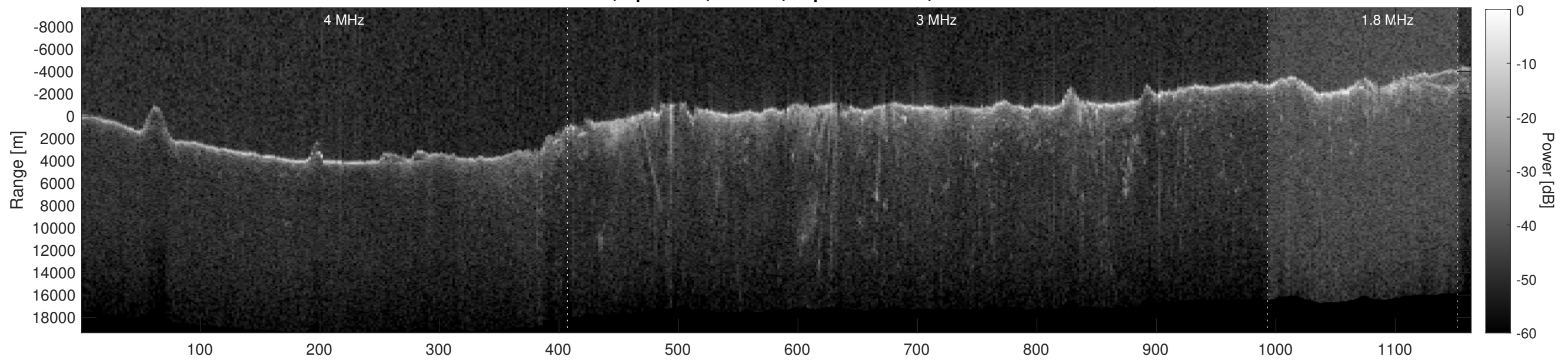
Orbit 2907, Depth-Corrected Cluttergram
