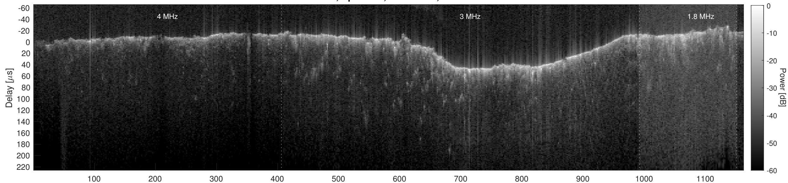
Orbit 2908, Cluttergram
