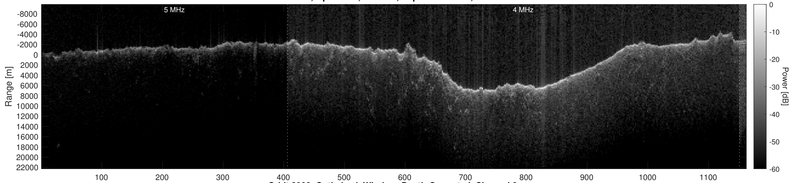
Orbit 2908, Optimized, Window, Depth-Corrected, Channel 2
