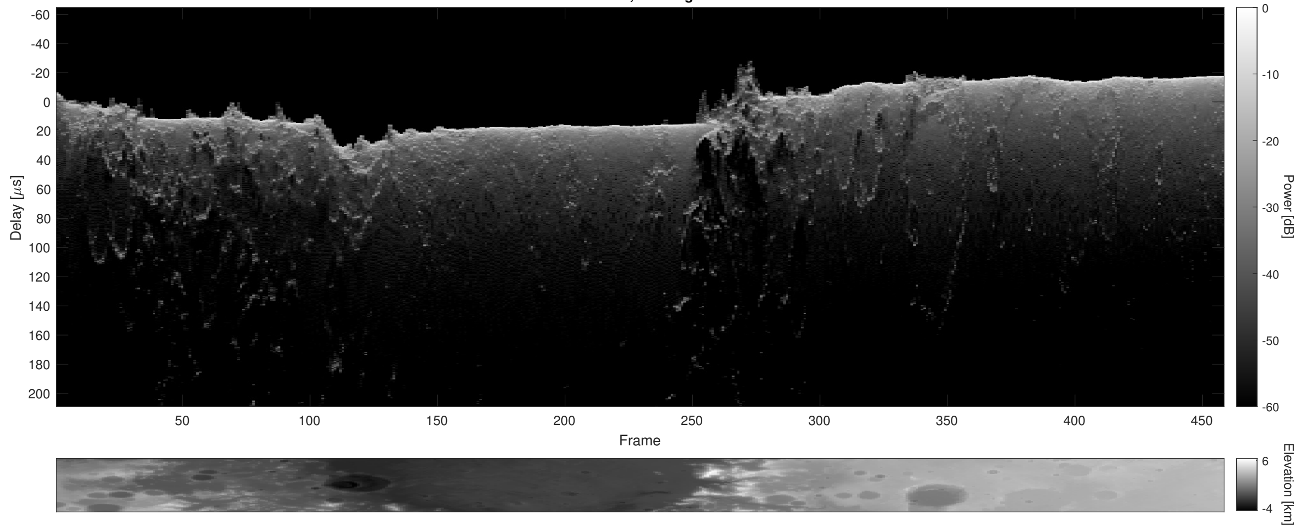
Orbit 2909, Cluttergram
